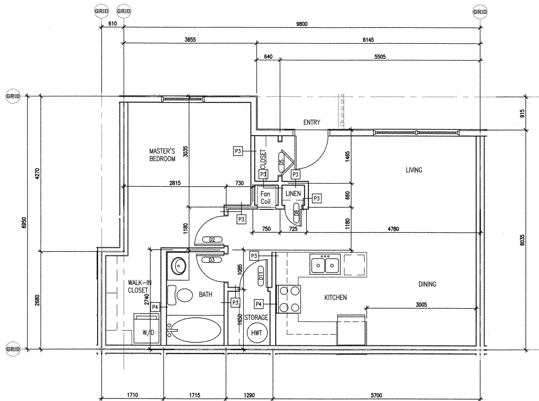
3 UNIT C ONE BEDROOM (AREA: 64.10 S.M.) A5.01 1:50
