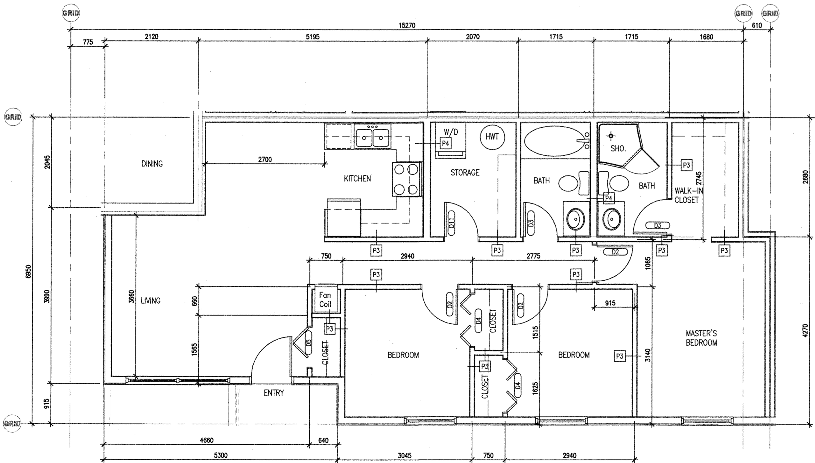
2 UNIT B THREE BEDROOM (AREA: 94.00 S.M.) A5.01 1:50
