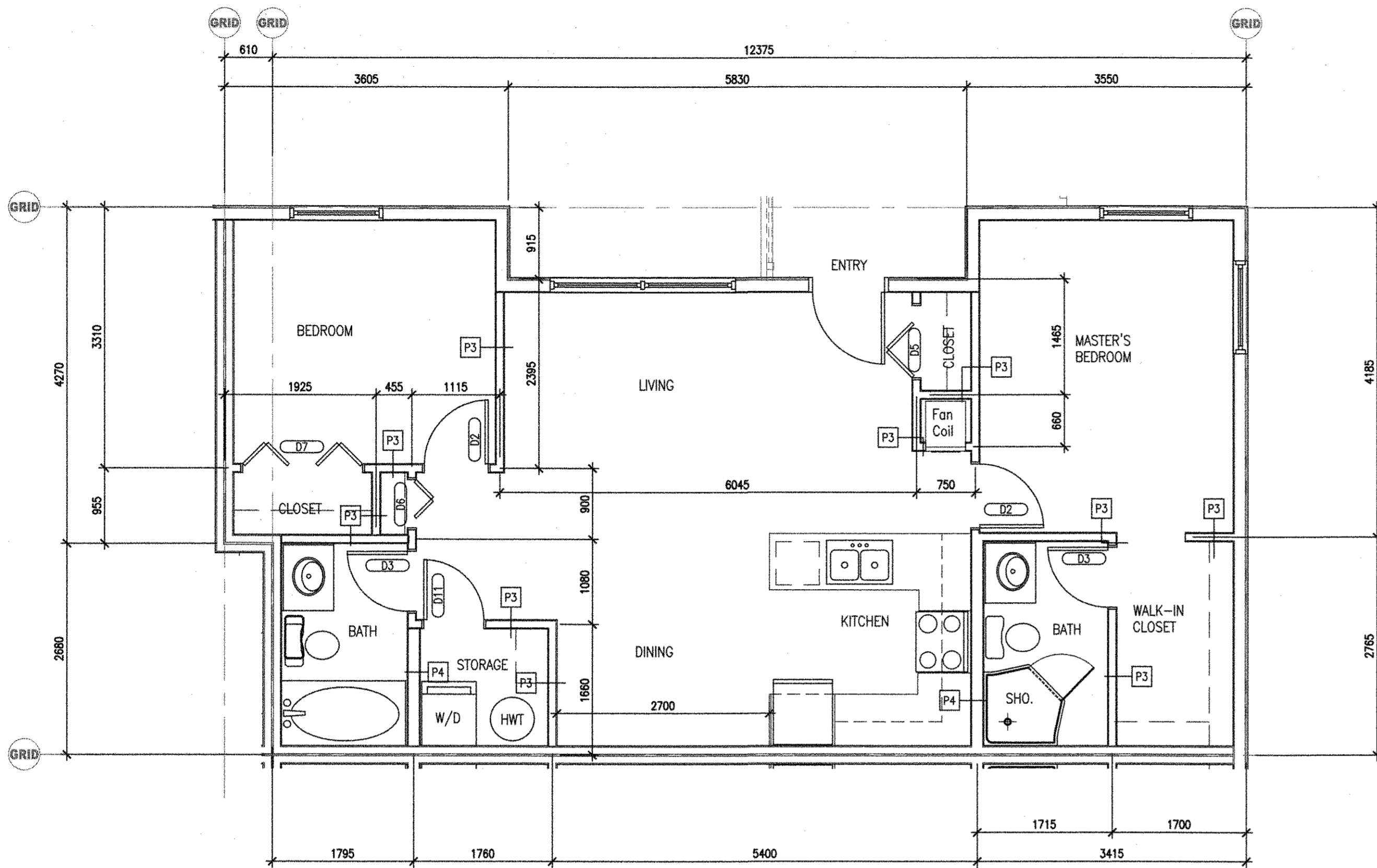
1 UNIT A TWO BEDROOM (AREA: 83.20 S.M.) A5.01 1:50
